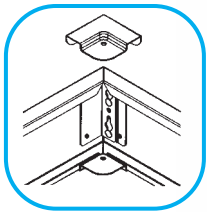
Securing top and bottom corner brackets
