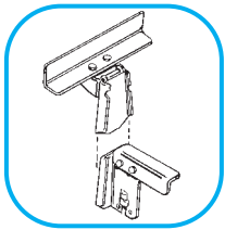
Wedge Lock™ Leg Design
